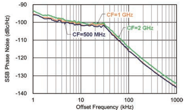
Example: SSB Phase Noise (Spectrum Analyzer/Signal Analyzer Common)
