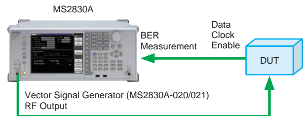
BER Measurement Setup Example (with MS2830A-020/021 installed)
